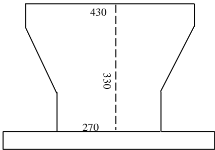
Hopper End View
